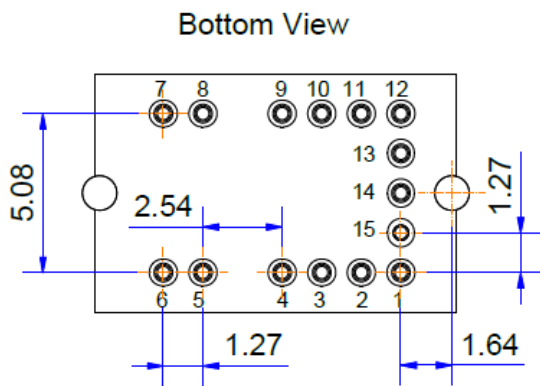
Figure 2: Module Bottom View (Dimensions in mm)
